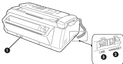
Figure 2-2 Rear view
